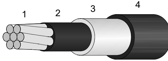
25 kV TREE PROOF AERIAL CABLE 4/0 AWG ALLOY 6201-T81 (107mm 2 ) 75° C BLACK
