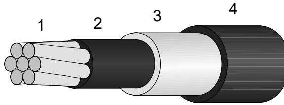
25 kV TREE PROOF AERIAL CABLE 3/0 AWG ALLOY 6201-T81 (85mm 2 ) 75° C BLACK
