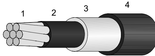
25 kV TREE PROOF AERIAL CABLE 2/0 AWG ALLOY 6201-T81 (67mm 2 ) 75° C BLACK Actual Alloy Area 155400 cmil (78.6 mm 2 )
