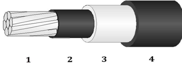
15 kV TREE PROOF AERIAL CABLE 2/0 AWG ALLOY 6201-T81 (67mm 2 ) 75° C BLACK
