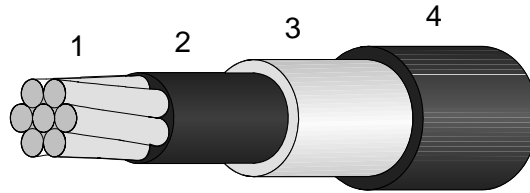
15 kV TREE PROOF AERIAL CABLE 1/0 AWG ALLOY 6201-T81 (54mm 2 ) 75° C BLACK
