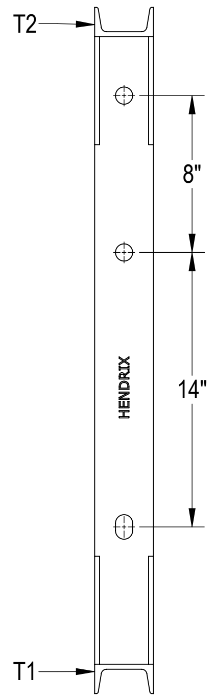
RIGHT VIEW
