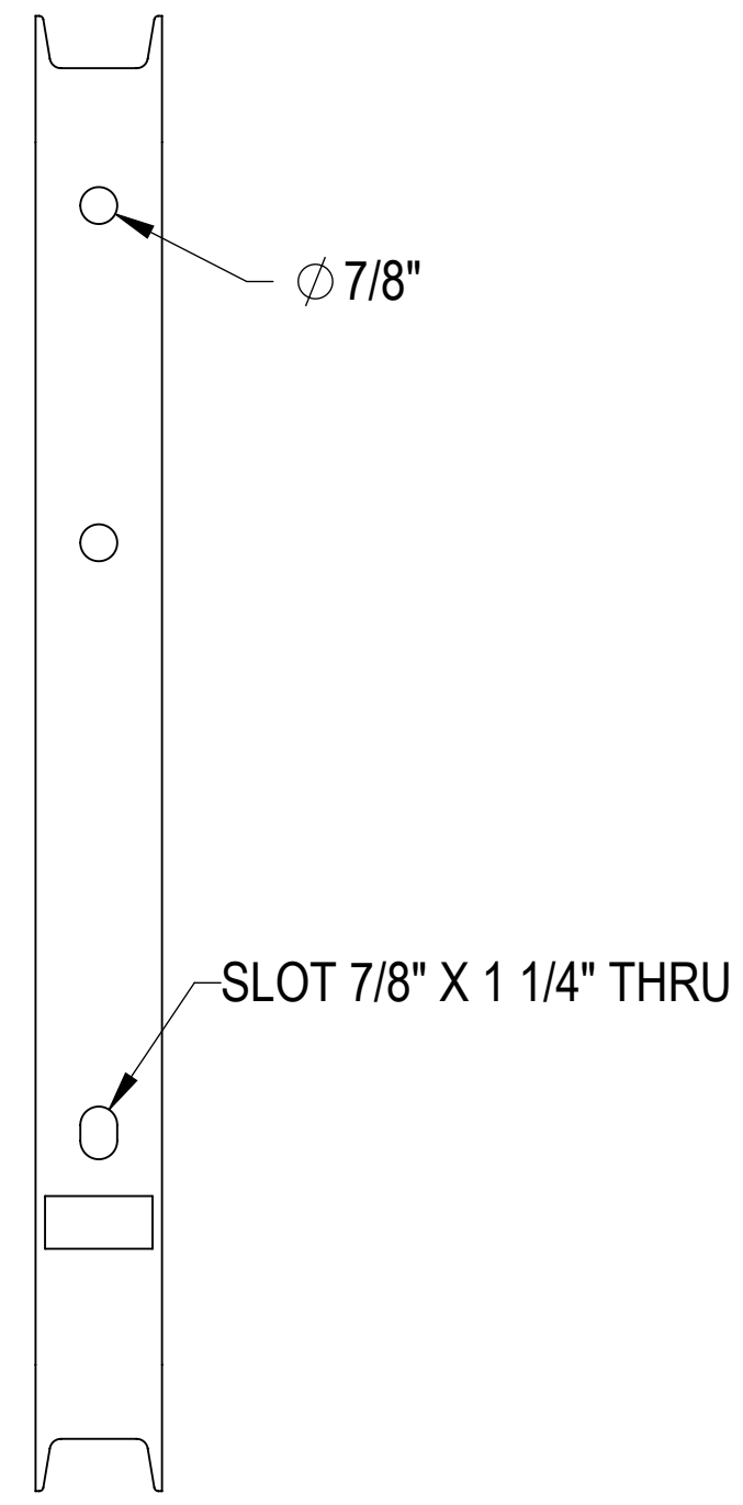
LEFT VIEW
