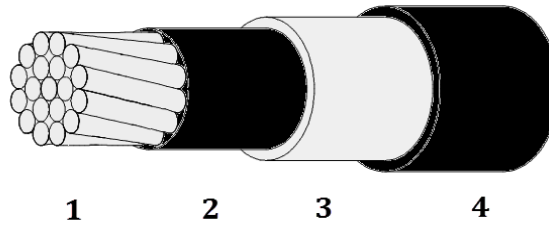
35 kV TREE PROOF AERIAL CABLE 477 KCM ACSR (242mm 2 ) 75° C BLACK
