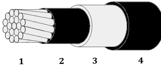
35 kV TREE PROOF AERIAL CABLE 397.5 KCM ACSR (201mm 2 ) 75° C BLACK
