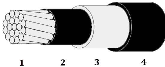
25 kV TREE PROOF AERIAL CABLE 397.5 KCM ACSR (201mm 2 ) 75° C BLACK
