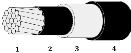
25 kV TREE PROOF AERIAL CABLE 336.4 KCM ACSR (170mm 2 ) 75° C BLACK
