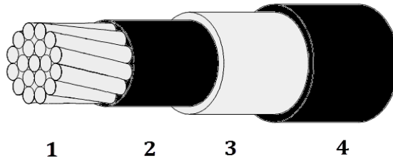
15 kV TREE PROOF AERIAL CABLE 266.8 KCM ACSR (135mm 2 ) 75° C BLACK
