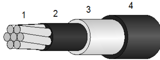
15 kV TREE PROOF AERIAL CABLE 4/0 AWG ACSR (107mm 2 ) 75° C BLACK
