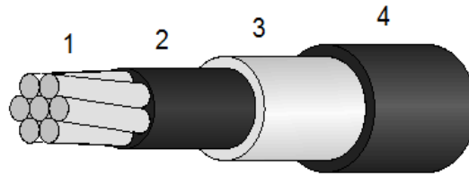
35 kV TREE PROOF AERIAL CABLE 3/0 AWG ACSR (85mm 2 ) 75° C BLACK
