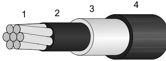
35 kV TREE PROOF AERIAL CABLE 2/0 AWG ACSR (67mm 2 ) 75° C BLACK
