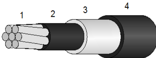
25 kV TREE PROOF AERIAL CABLE 1/0 AWG ACSR (54mm 2 ) 75° C BLACK
