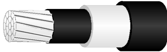
15 kV AERIAL CABLE 636 KCM AAC (322mm 2 ) 75° C BLACK
