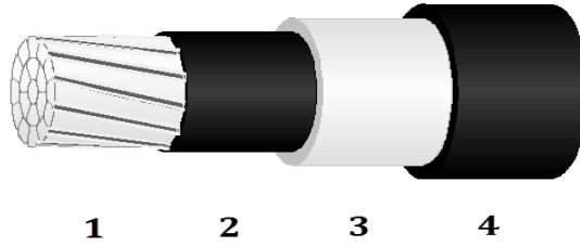
25 kV AERIAL CABLE 556.5 KCM AAC (282mm 2 ) 75° C BLACK
