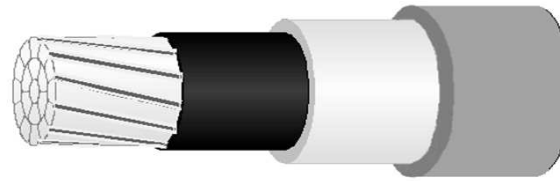
1 2 3 4 69 kV AERIAL CABLE 397.5 KCM AAC (201mm 2 ) 75° C GRAY
