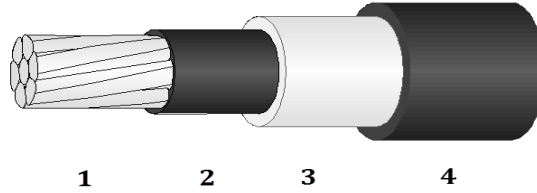
25 kV AERIAL CABLE 3/0 AWG AAC (85mm 2 ) 75° C BLACK
