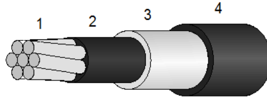
35 kV AERIAL CABLE 1/0 AWG AAC (54mm 2 ) 75° C BLACK
