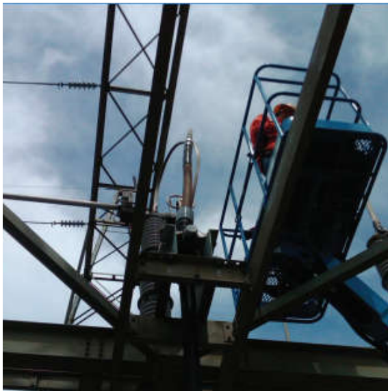
Termination removed and cable exposed and ready to be re-prepped so termination can be replaced.
