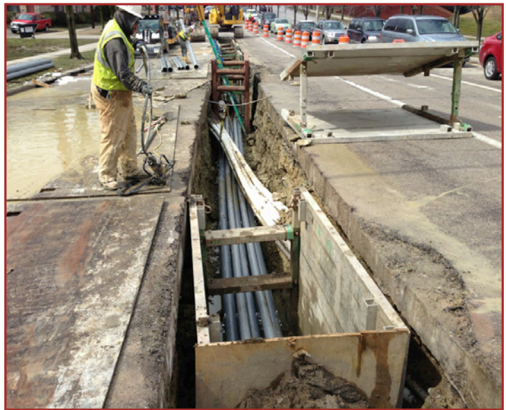
Construction of concrete encased ducts on Martin Luther King Jr. Blvd.
