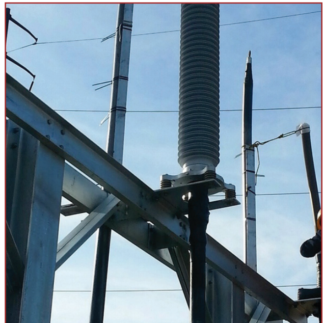
Newly installed Tyco OHVT-145 termination
